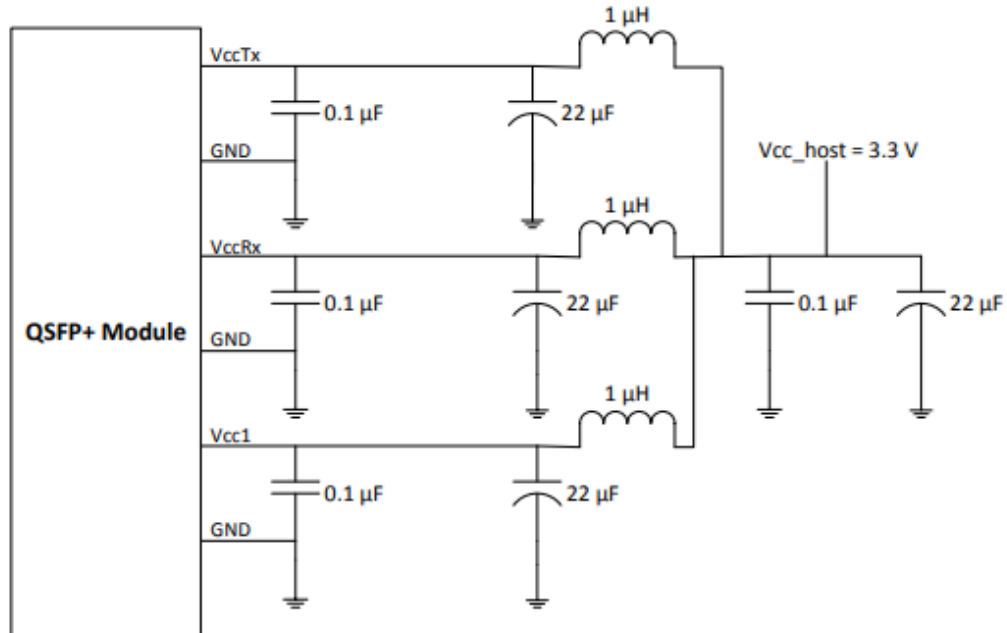
FIGURE 5-4 RECOMMENDED HOST BOARD POWER SUPPLY FILTERING
