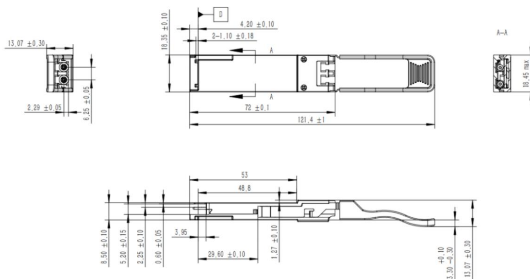
Figure 2. Mechanical Dimensions
