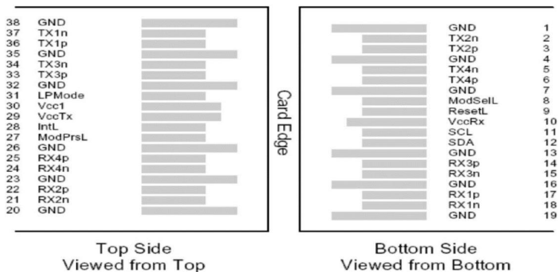
Figure 1 QSFP28-compliant 38-pin connector (per SFF-8679)
